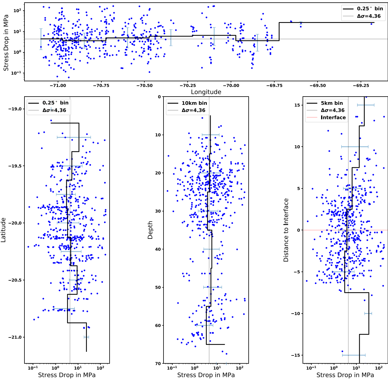
Figure 9. Stress drop variation in the spatial domain. The top panel shows stress drop estimates versus longitude. Below, the stress drop distribution is shown from north to south, against depth and relative to the plate interface from left to right, respectively. The binning interval is given in the plot legends. No smoothing is applied. The solid line traces the median value computed for each bin separately. To indicate the spread of values in each bin we plot a blue error bar from the median of the upper to the median of the lower half of values, which are separated by the overall median in the bin. In all plots the median of the entire data set ( \Delta\sigma = 4.36 MPa) is underlain as a gray line. In the last panel positive distance values refer to events located above the plate interface (red line), negative values to events below it.
